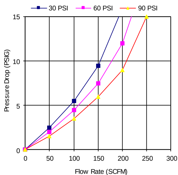
AF4000-06 Series Filter Flow Rate VS Pressure Drop @ 30, 60, 90 PSI Supply Pressure
