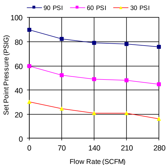
AW5000 Series Filter Regulator Flow Rate VS Set Point Pressure Supply Pressure 100 PSI
